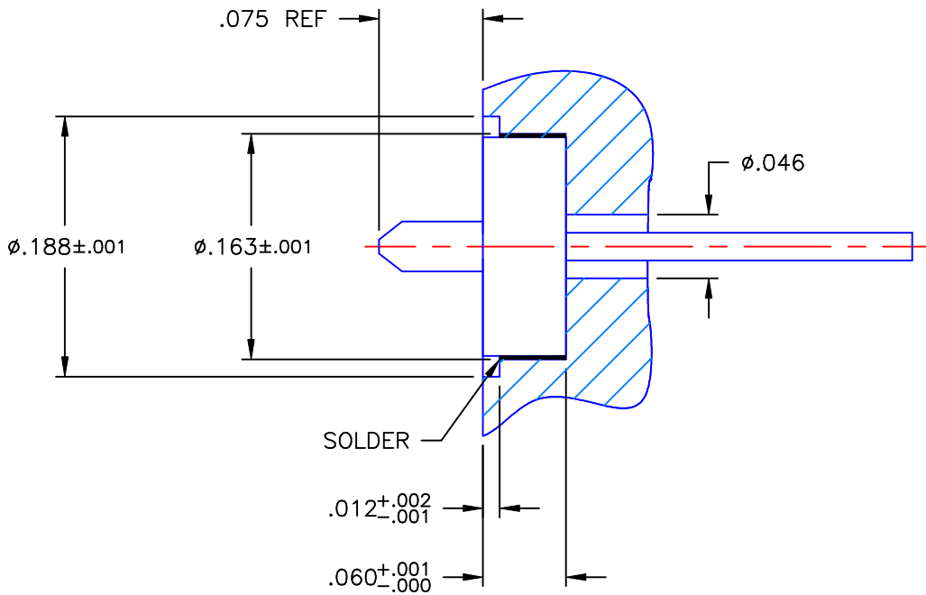
RECOMMENDED MOUNTING
